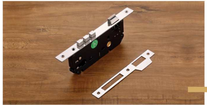
Lock Body Size in mm : 45 x 85 / 50 x 85 / 60 x 85 Finish : Black Satin / PVD Black
