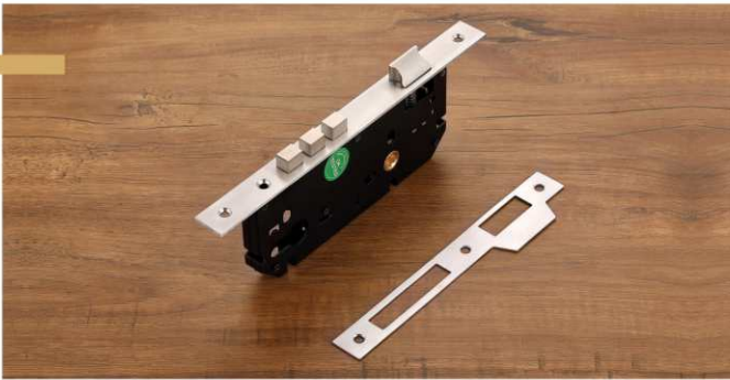
Lock Body Size in mm : 45 x 85 / 50 x 85 / 60 x 85 Finish : S.S.
