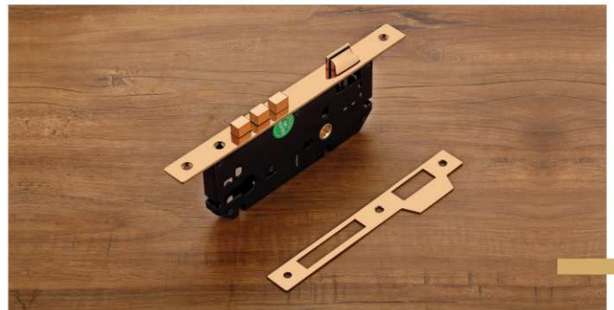
Lock Body Size in mm : 45 x 85 / 50 x 85 / 60 x 85 Finish : PVD R.G.
