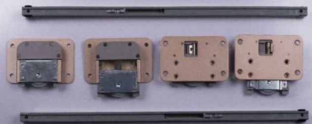
CL-2700 (Wardrobe Sliding universal Door Runner)
