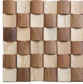
2107 - Size: 275 mm x 275 mm Thickness: 10 mm, Weight: 330 grm
